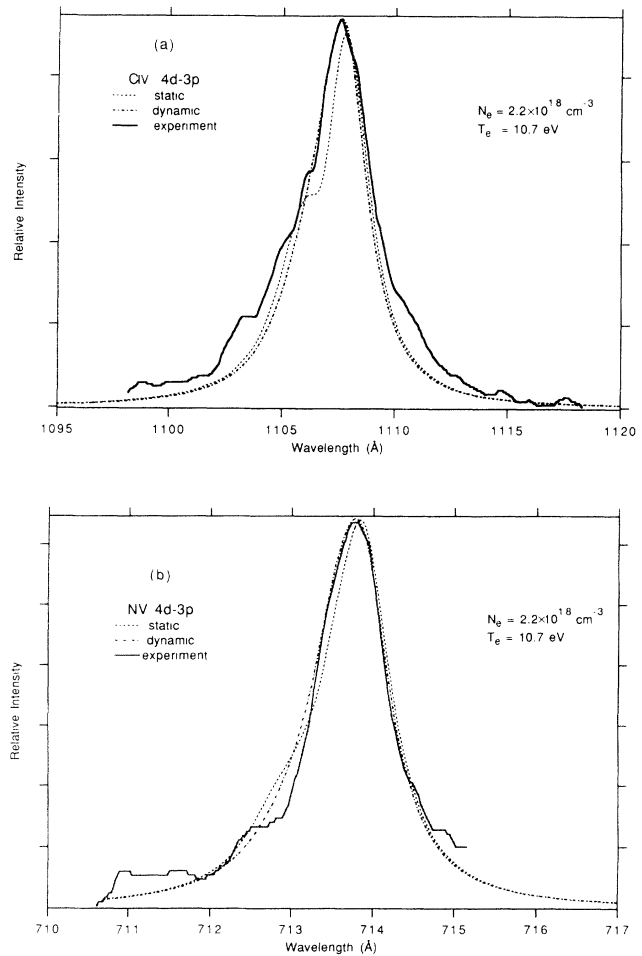
FIG. 2. (a) The theoretical C IV 4d-3p dipole-allowed transition profile compared to the experiment. The plasma conditions are the same as in Fig. 1, but the theoretical profiles have been convolved with the second order apparatus function (approximately 0.9 Å FWHM) for comparison with the experiment. The data points are indicated by the solid line and the two convolution calculations are labeled as in Fig. 1. The ion dynamic profile is seen to be in good agreement with the experiment. (b) The theoretical N V 4d-3p profiles compared to the experiment. The plasma conditions are the same as in Fig. 1, but the theoretical curves have been convolved with the fourth order apparatus function (approximately 0.45 Å FWHM) for comparison with the experiment. The data points are indicated by the solid line and the calculation is labeled as in Fig. 1. Note the good agreement of the theory with the ion dynamics profile.
