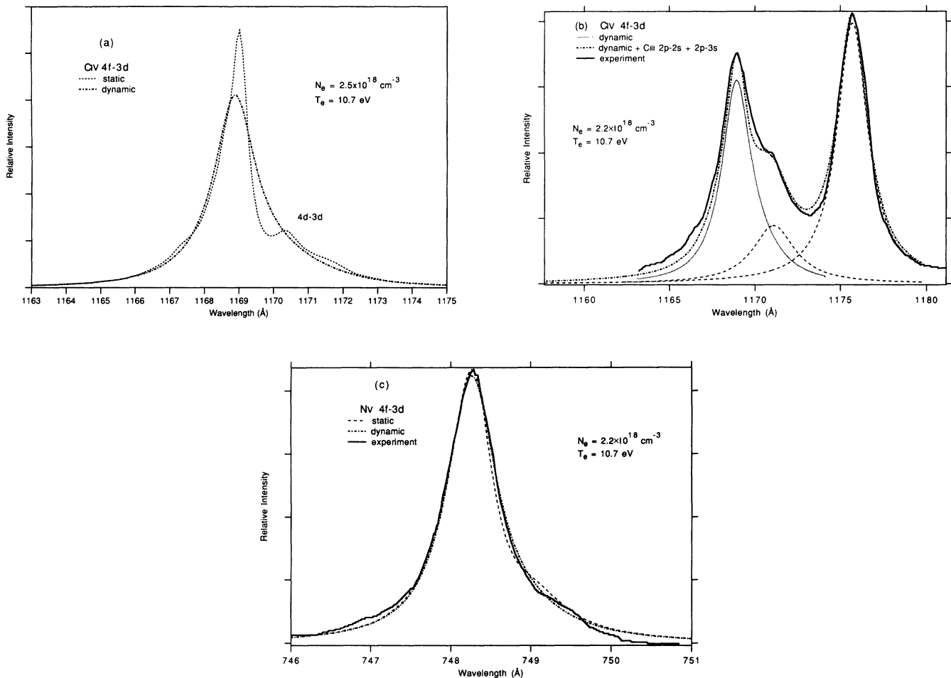
FIG. 3. (a) The theoretical line shape for the lithiumlike carbon C IV, dipole-allowed 4f-3d transition at 1169 \text{ \AA} and the associated dipole-forbidden 4d-3d transition at 1171.5 \text{ \AA} . The line profiles are displayed as relative intensity versus wavelength in angstroms and the dot-dashed curve is the theory with ion dynamics effects while the dashed curve is the static microfield calculation. The plasma conditions are the same as for the preceding figures, with electron density N_e = 2.2 \times 10^{18} \text{ cm}^{-3} and temperature T_e = 10.7 \text{ eV} . The merging and complete disappearance of the forbidden transition when ion dynamics is taken into account is an important feature of this profile. (b) The comparison of the theoretical C IV 4f-3d profile to the experiment. The plasma conditions are the same as in (a), but the theoretical curves have been convolved with the second order apparatus function (approximately 0.9 \text{ \AA} FWHM) for comparison with the experimental data. The experimental points are indicated by the solid line and the calculations are labeled as in (a). Included also is the contribution of the C III 2p^2-2p2s line at 1176 \text{ \AA} in second order and the 585 \text{ \AA} C III 2p3s-2p^2 line at 1171 \text{ \AA} in fourth order, individually treated as Lorentzian contributions and shown as dashed lines. The total of the theory including ion dynamics and these two lines is represented by the dot-dashed line. This total line shape can be seen to be in good agreement with the data points. (c) The comparison of the theory and experiment for the N V 4f-3d transition at 748.2 \text{ \AA} . The theory includes a convolution with the apparatus profile (approximately 0.45 \text{ \AA} FWHM) for the fourth order dispersion. The line profile is presented as relative intensity versus wavelength in angstroms, the data points are indicated by the solid line, the dot-dashed curve is the theory with ion dynamics effects while the dashed curve is the static microfield calculation. The plasma conditions are the same as in the preceding figures. Good agreement with the theory including ion dynamics can be seen.
